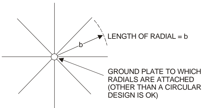
Figure 3-16. Radials.
