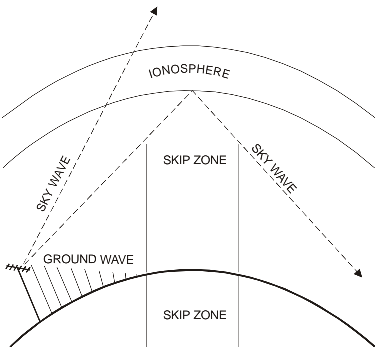
Figure 2-2. HF Propagation.
