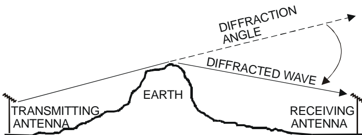
Figure 2-5. VHF Diffraction.
