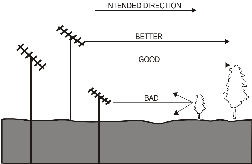
Figure 3-5. Antenna Obstacles.
