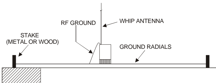
Figure 3-17. Equipment Configuration.
