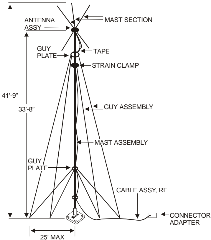
Figure 4-5. OE-254 Antenna.
